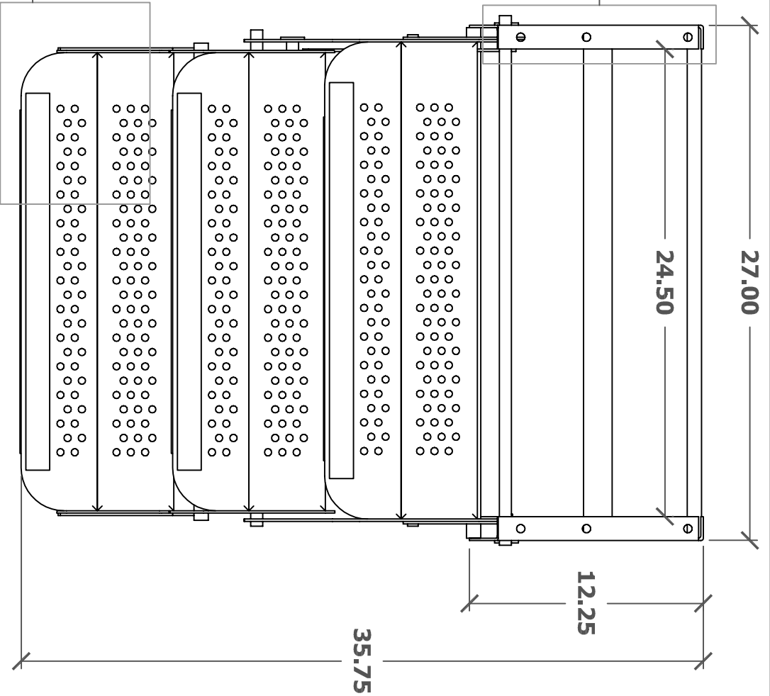
Top View
